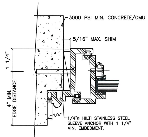
2A ALTERNATE MOUNT TO CONCRETE/CMU
