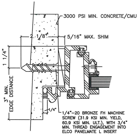
2 MOUNT TO CONCRETE/CMU
