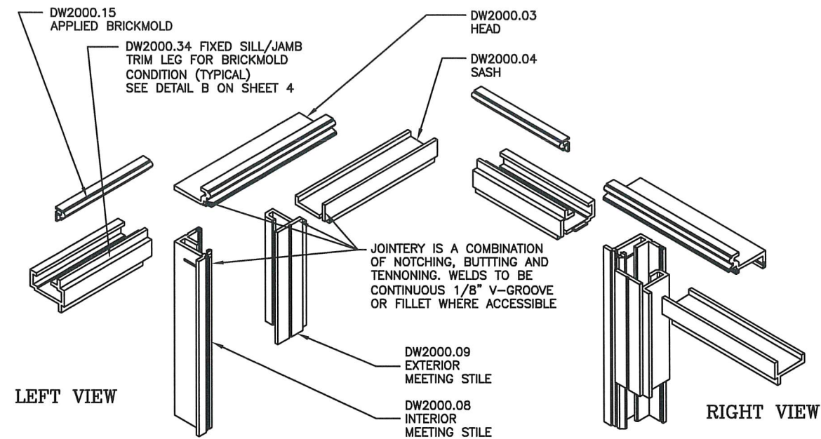
1 EXPLODED ISOMETRIC VIEW TYPICAL FIXED TO CASEMENT MEETING RAIL SCALE: NTS
