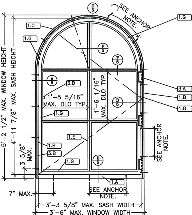
2 ROUND TOP EXTERIOR ELEVATION
