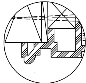
3 STANDARD BRICK MOLDING
