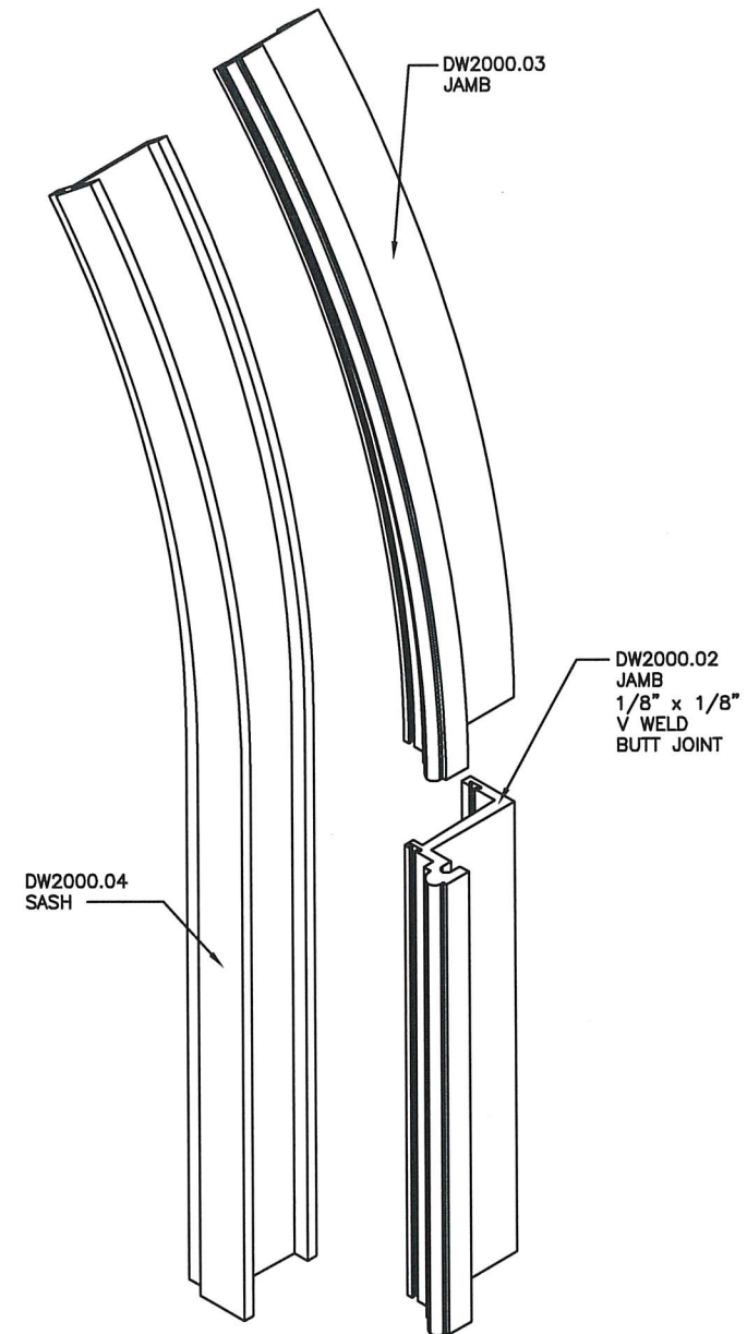
4 EXPLODED ISOMETRIC VIEW TYPICAL CURVED HEAD TO JAMB SCALE: NTS
