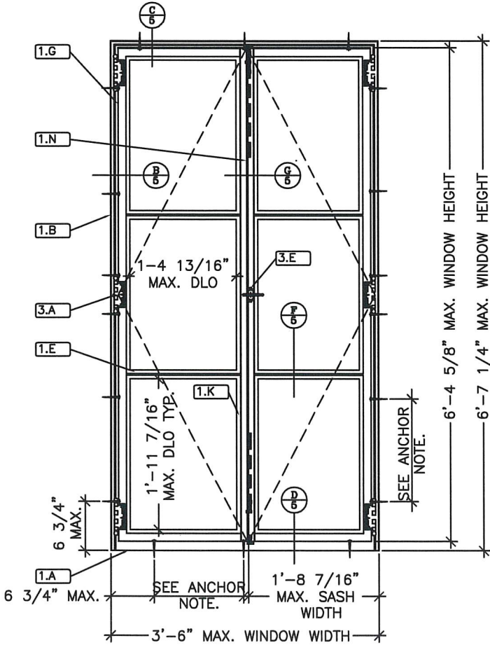
4 DOUBLE CASEMENT EXTERIOR ELEVATION
