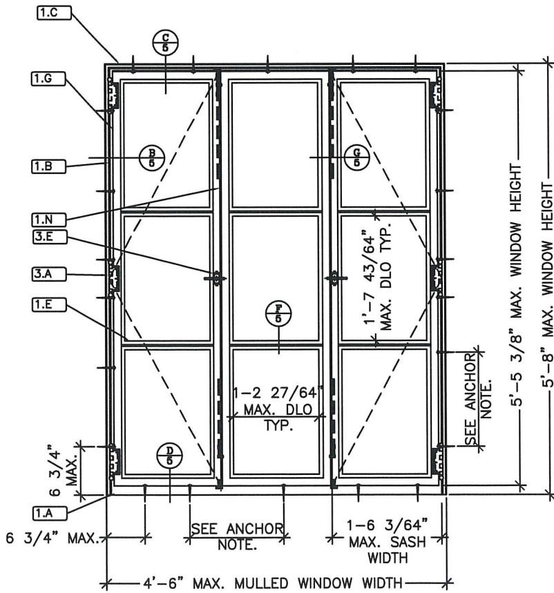
5 DOUBLE CASEMENT WITH FIXED CENTER LITE EXTERIOR ELEVATION
