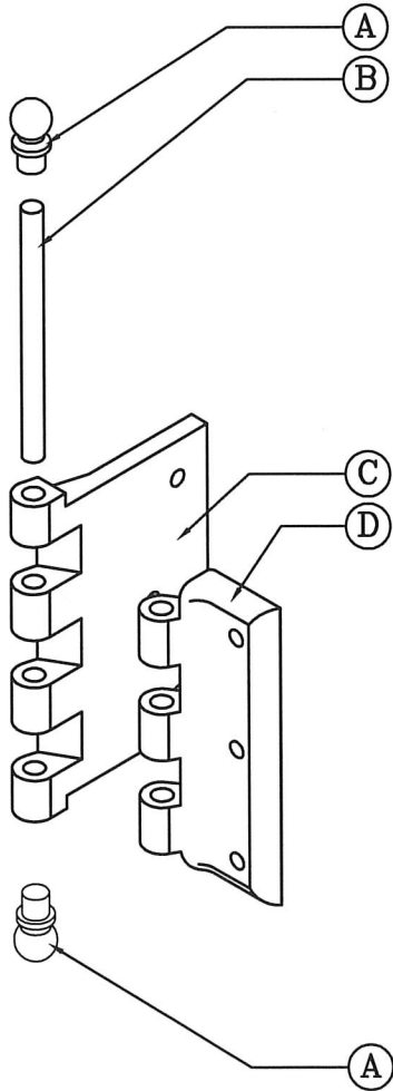
2 EXPLODED 4" HINGE
