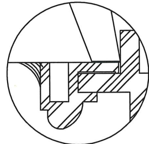
4 APPLIED BRICK MOLDING
