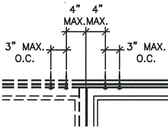
A MULLION AND MTG STILE ENDS, HEAD AND SILL ANCHOR CLUSTER DETAIL
