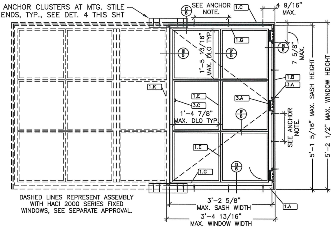
1 CASEMENT WITH FIXED WINDOW EXTERIOR ELEVATION
