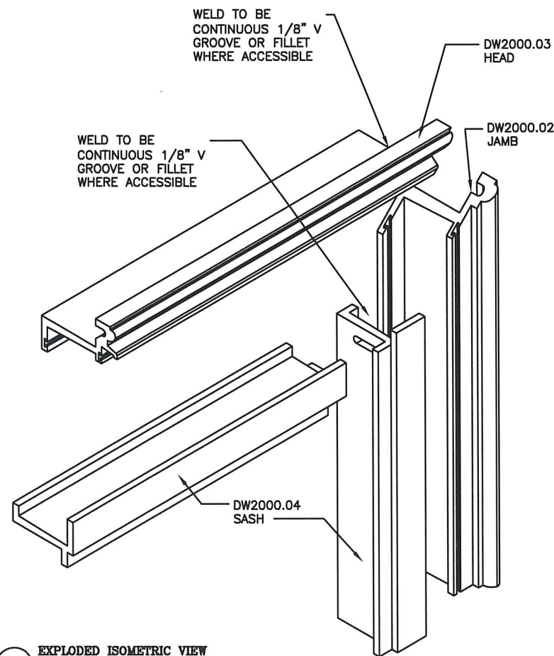
3 EXPLODED ISOMETRIC VIEW ALTERNATE CORNER SCALE: NTS
