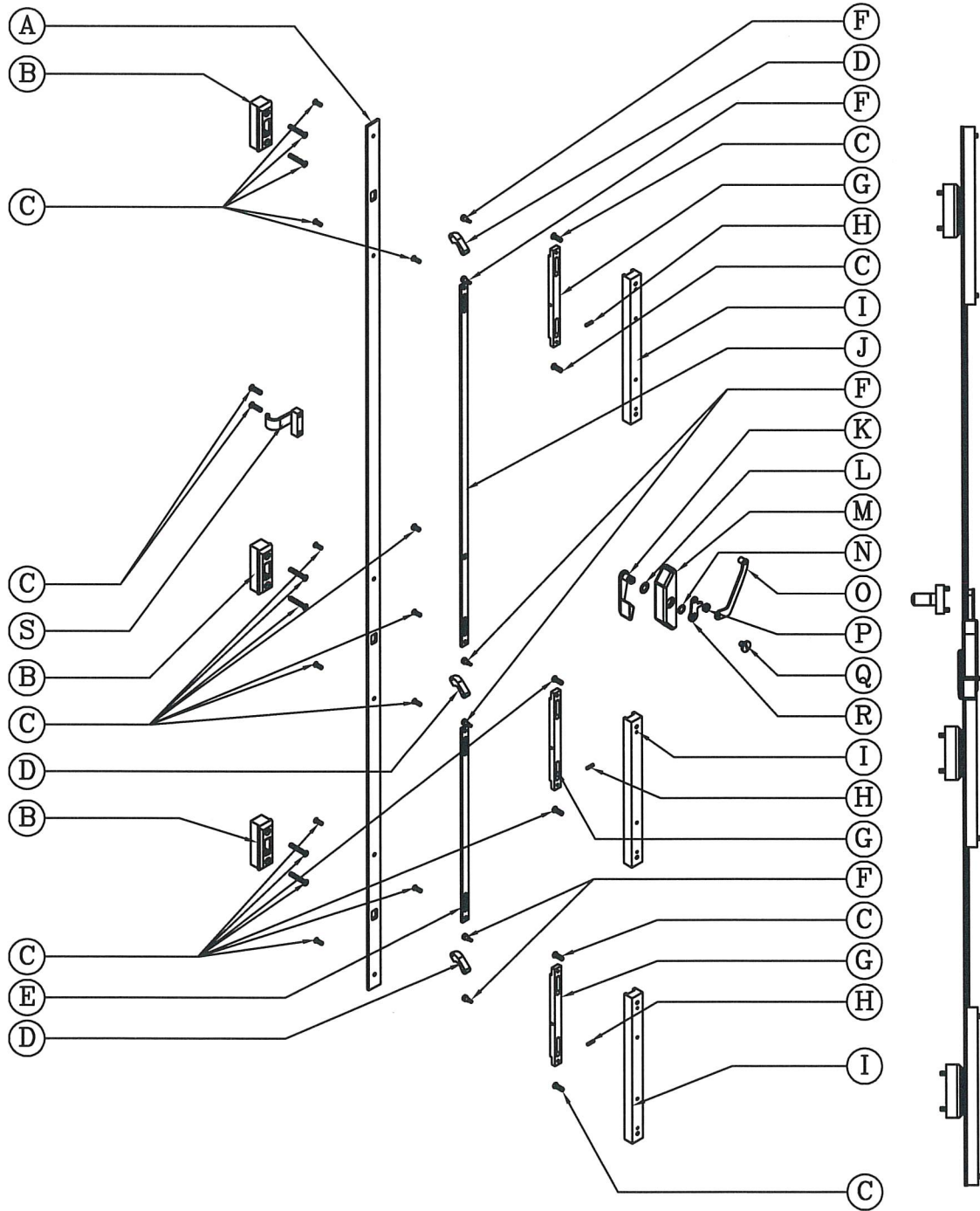
EXPLODED
